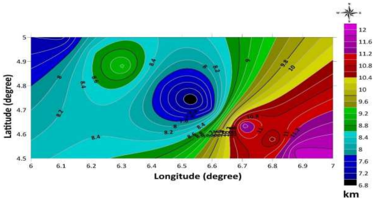
Figure 10: Sedimentary thickness along profile line-2
