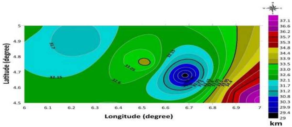
Figure 8: Crustal thickness along profile line-1
