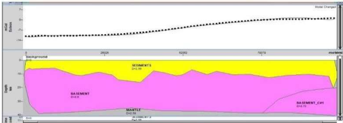
Figure 9: Crustal Modelling along profile line-2
