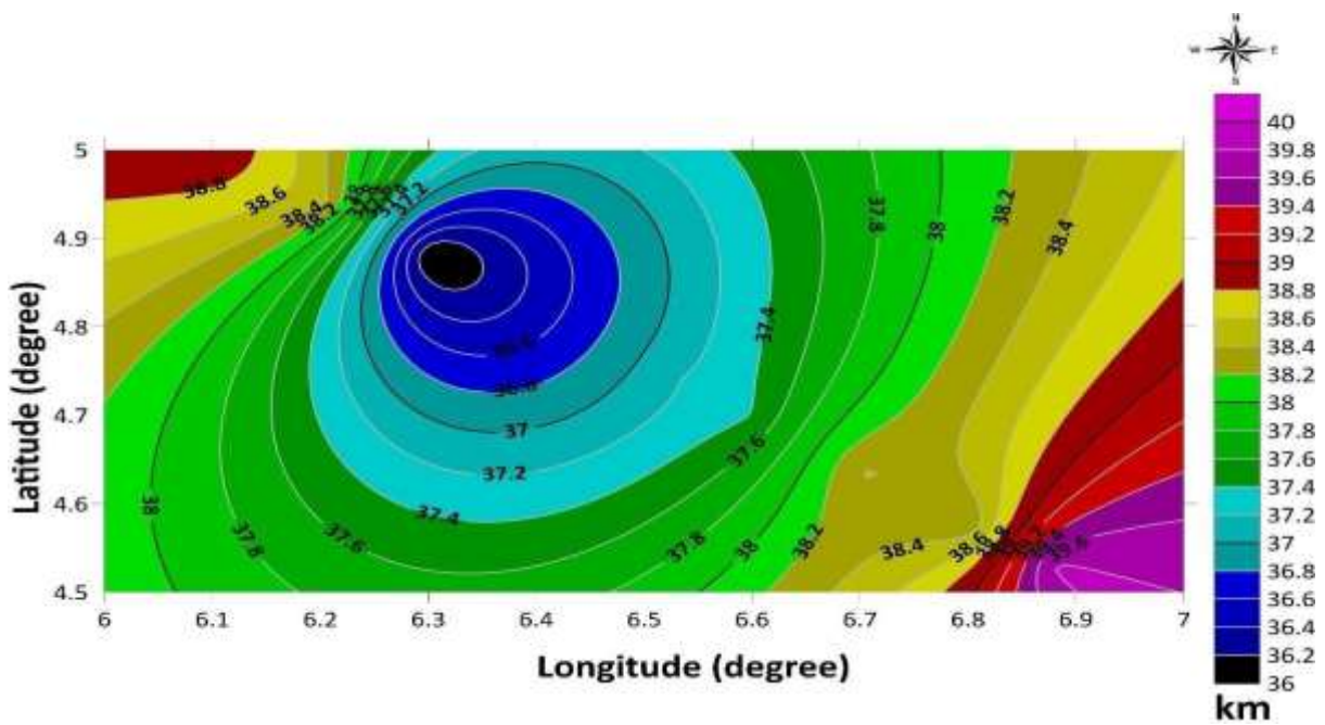
Figure 11: Crustal thickness along profile line-2
