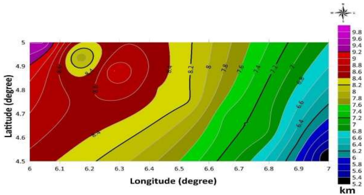
Figure 7: Sedimentary thickness along profile line-1
