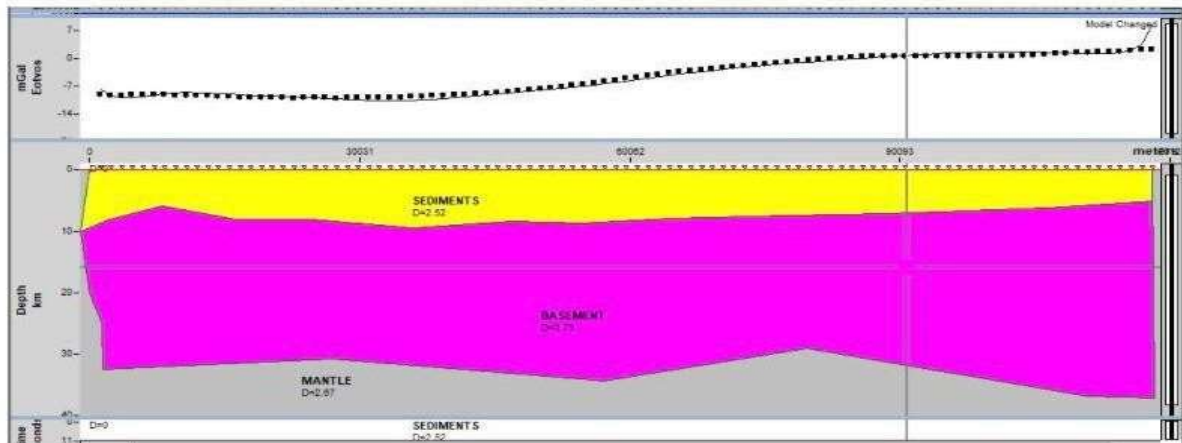
Figure 6: Crustal Modelling along profile line-1
